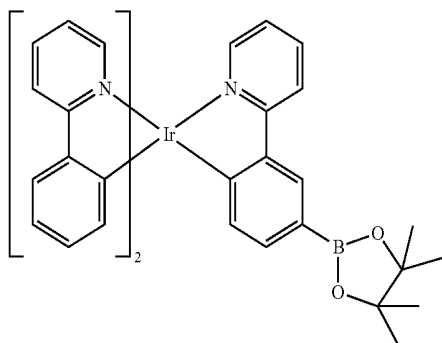
Synthesis of Irppy Intermediate
