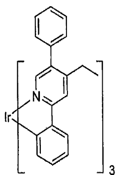
Compound 22
