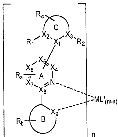
Formula II
