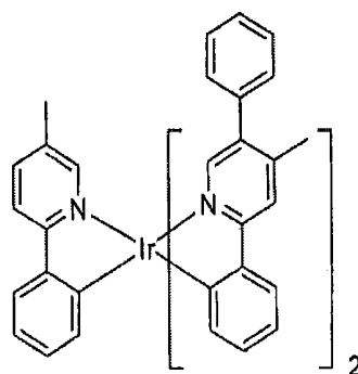
Compound 34
