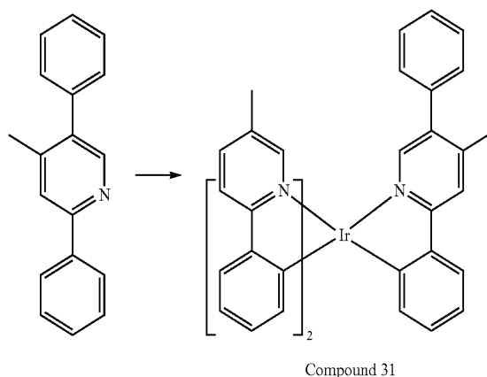
Compound 31
