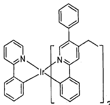
Compound 30
