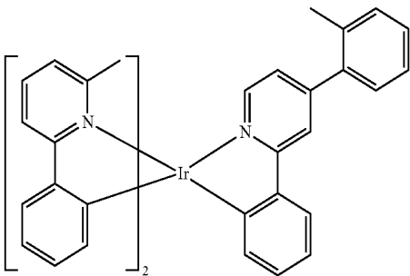
Compound 28
