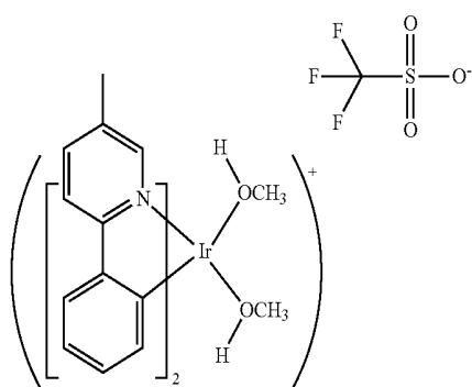
Synthesis of Ir Triflate
