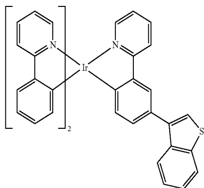
Compound 6
