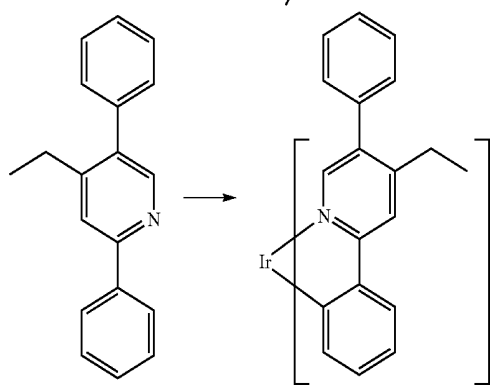
Compound 22
