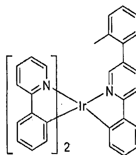
Compound 25
