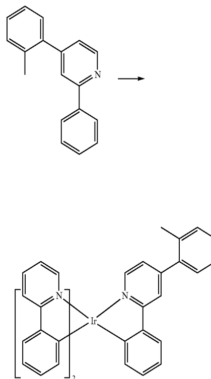
Compound 27
