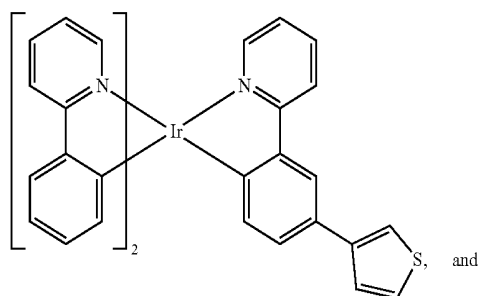
Compound 5
