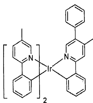
Compound 31
