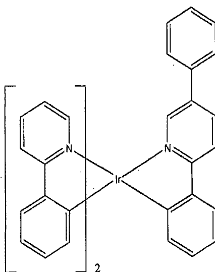
Compound 2
