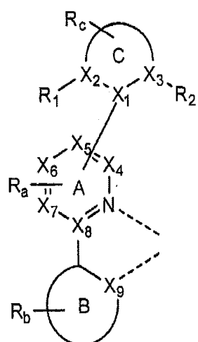
Formula I
