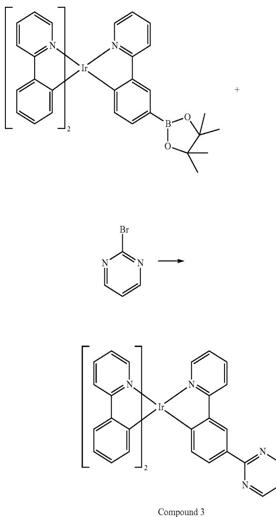
Compound 3
