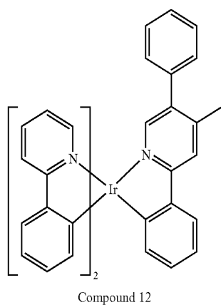
Compound 12
