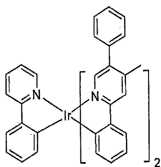
Compound 29
