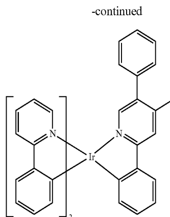
Compound 12
