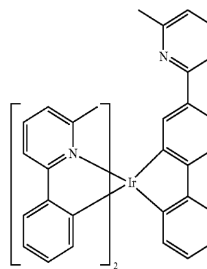
Compound 13
